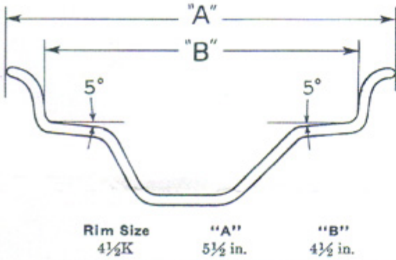
Kelsey-Hayes Wheel with Wide Base Semi-Drop Center Rim
