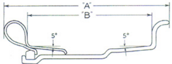
Kelsey-Hayes Wheel with Wide Base Rim
