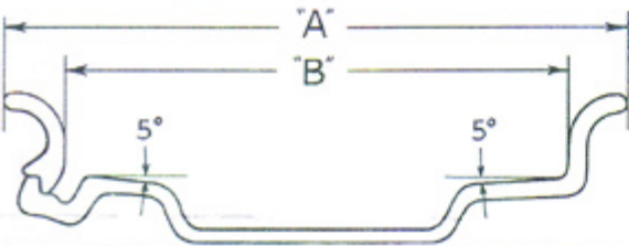
Kelsey-Hayes Wheel with Wide Base Rim
